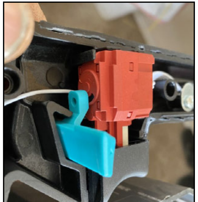
Figure 17b—Properly seated switch assembly.
