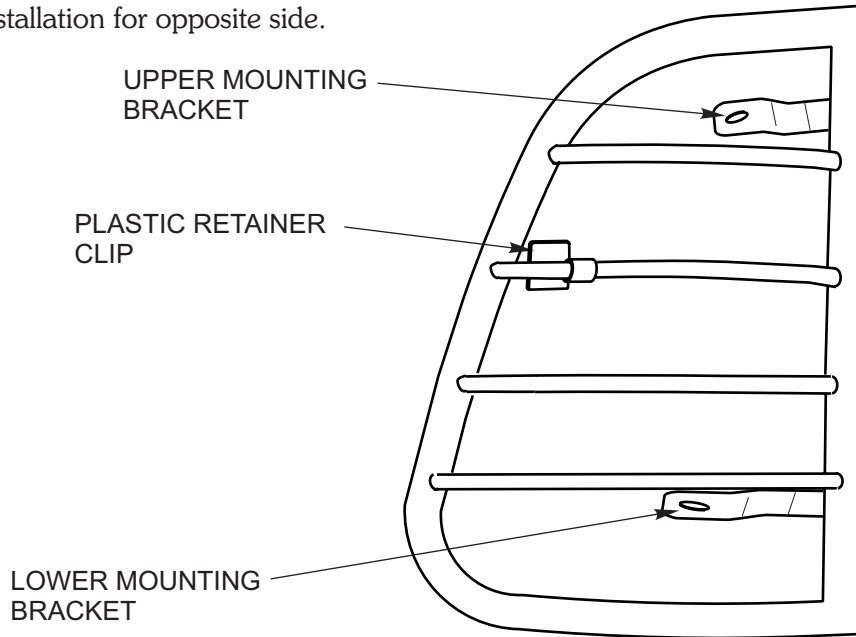
DRIVER SIDE SHOWN, PASSENGER SIDE OPPOSITE
