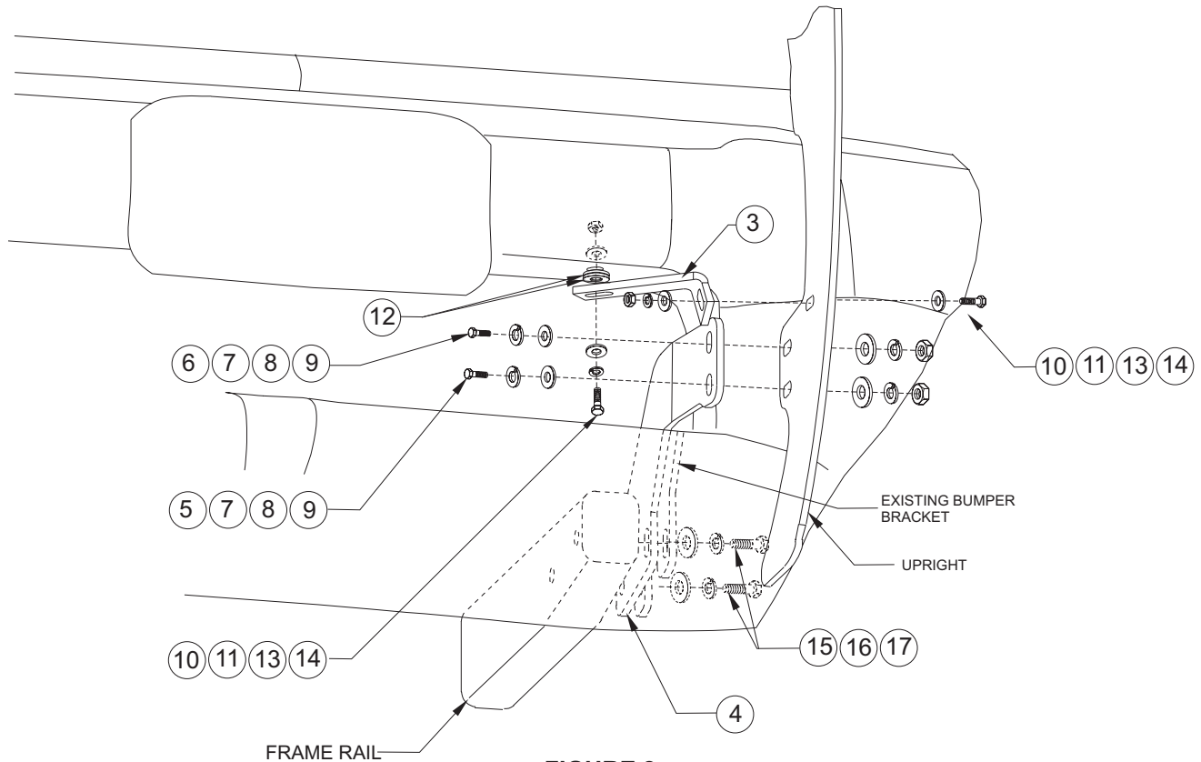
FIGURE 2 INSTALLATION VIEW OF DRIVER SIDE. PASSENGER SIDE OPPOSITE
