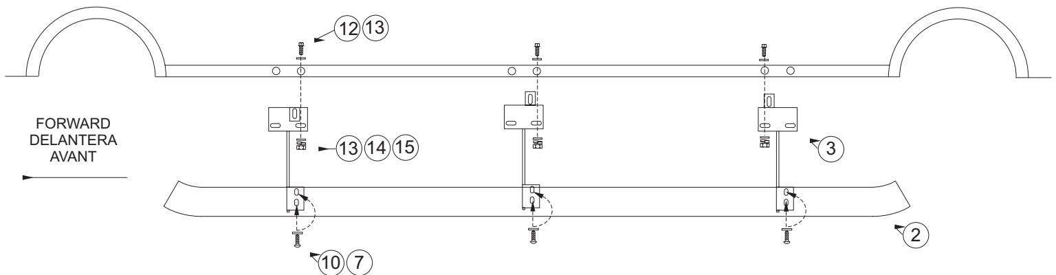
FIGURE 1 INSTALLATION VIEW OF DRIVER SIDE SHOWN, PASSENGER SIDE OPPOSITE FIGURA 1 VISTA DE LA INSTALACIÓN DEL LADO DEL CONDUCTOR OPUESTO AL LADO DEL ACOMPAÑANTE FIGURE 1 ILLUSTRATION: DRIVER SIDE, PASSENGER SIDE OPPOSITE
