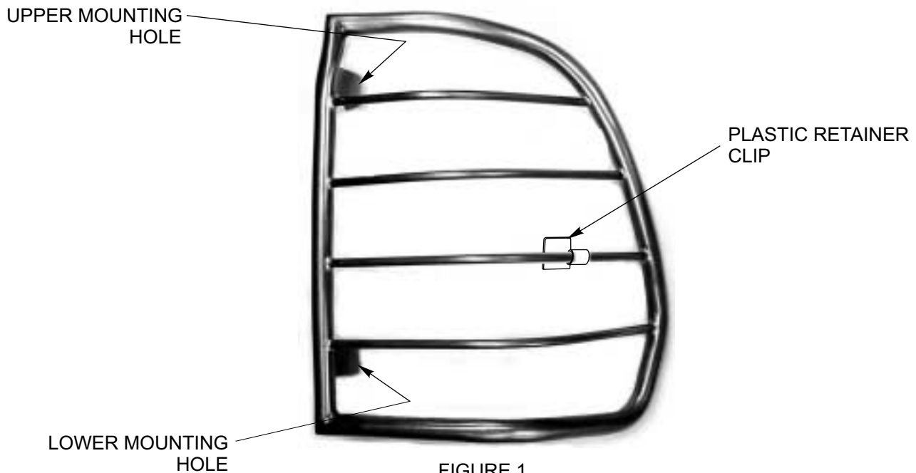
FIGURE 1 DRIVER SIDE TAILLIGHT GUARD SHOWN
